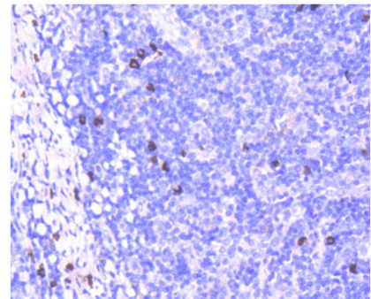
Fig. 2. Immunohistochemical analysis of paraffin-embedded human tonsil tissue using anti-CD63 antibody. Counter stained with hematoxylin.
