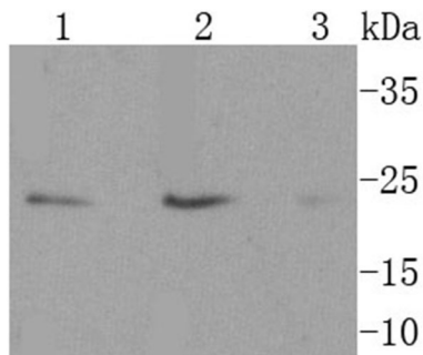
Fig. 1. Western blot analysis of CD63 on different lysates using anti-CD63 antibody at 1/1,000 dilution. Positive control: Lane 1: HL60; Lane 2: THP-1; Lane 3: NIH/3T3
